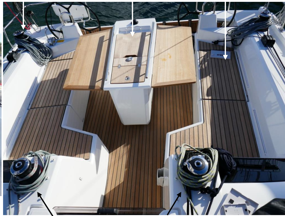
2 Self tailing coachroof winches (H40.2 STA). Standard
